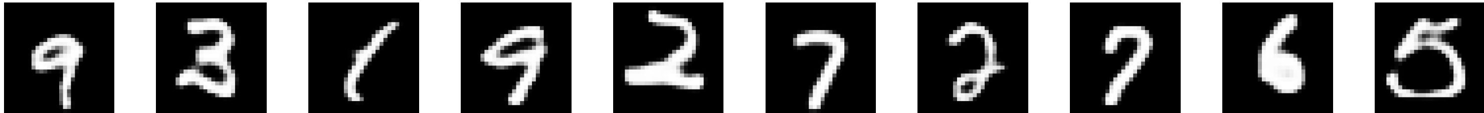
Conv2DTranspose
