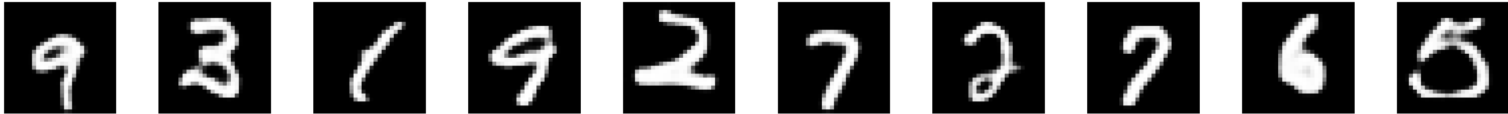
Conv2DTranspose
